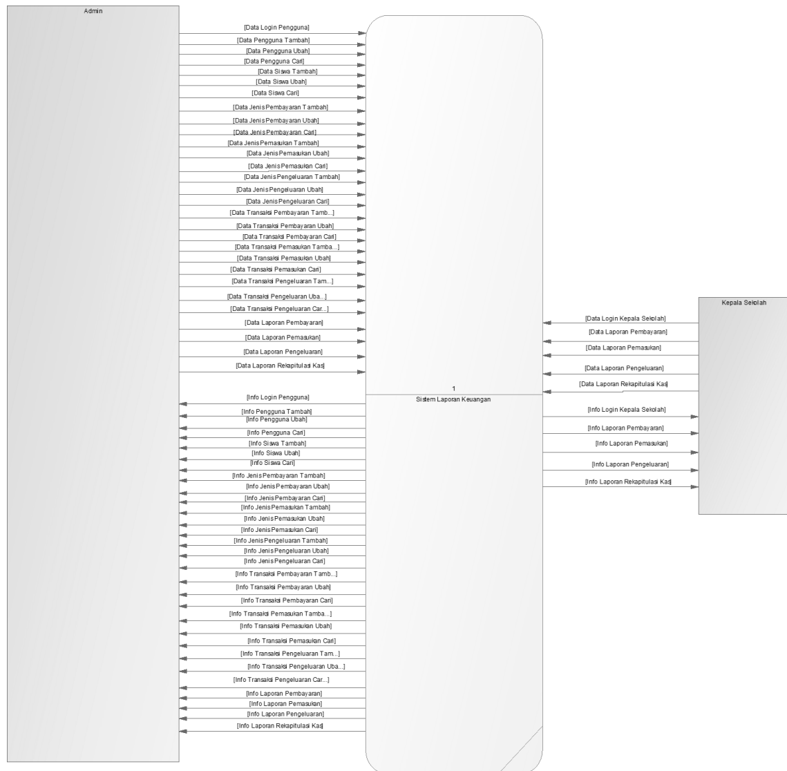
Gambar 1. Context Diagram
