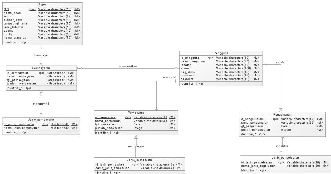
Gambar 2. Conceptual Data Model
